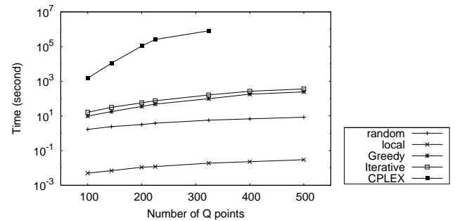
Figure 15: Running time of different replica selection algorithms.
