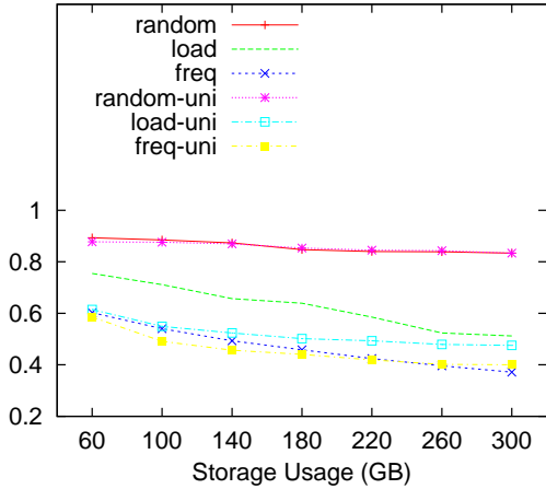
Figure 13: Performance of hard-quality replica selection algorithms under different query distributions.
