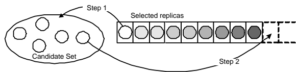
Figure 6: Replica replacement in Iterative Greedy.
