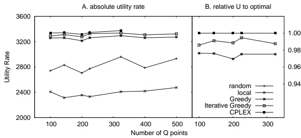
Figure 14: Optimality of replica selection algorithms.
