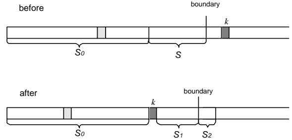
Figure 11: Replica selection upon query rate change.
