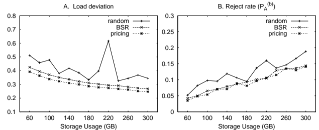
Figure 18: Performance of load balancing methods.
