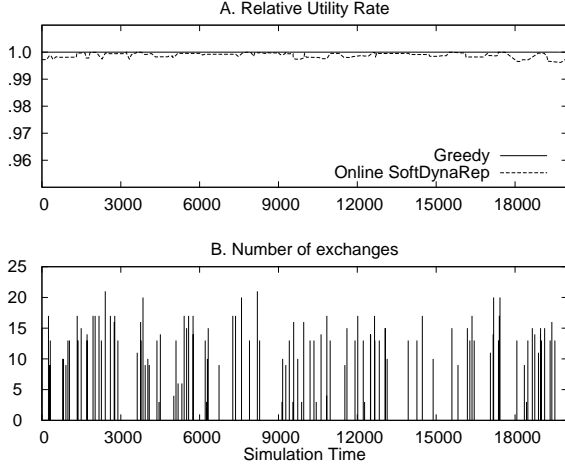
Figure 19: Performance of SOFTDYNAREP.
