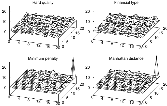
Figure 16: Frequency of replicas chosen by Greedy in a 20 \times 20 quality space.
