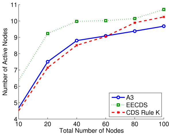
Figure 3: Active nodes vs. network density.
