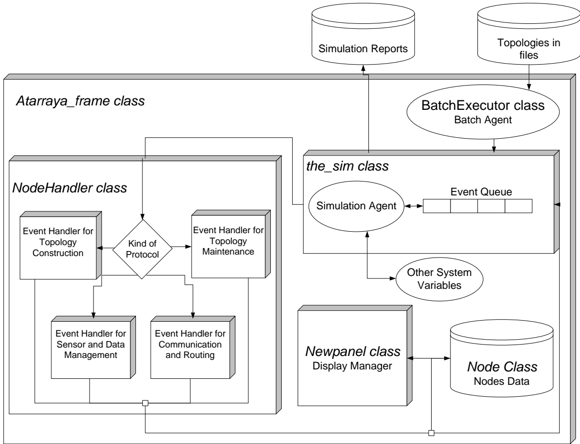
Figure 1: Atarraya's functional components.
