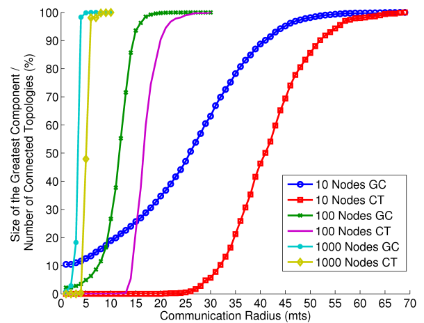
Figure 2: The giant component experiment.
