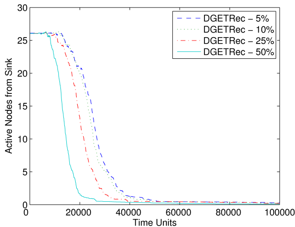
Figure 4: Example of a test of sensitivity of topology maintenance protocols in Atarraya
