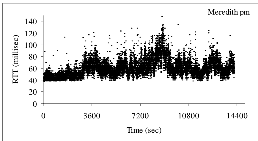
Figure 2 - Time vs RTT for Meredith pm dataset
