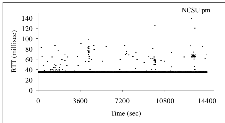
Figure 4 - Time vs RTT for NCSU am dataset
