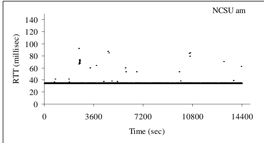
Figure 3 - Time vs RTT for NCSU am dataset
